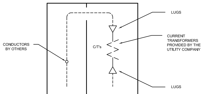
ONE LINE DIAGRAM
