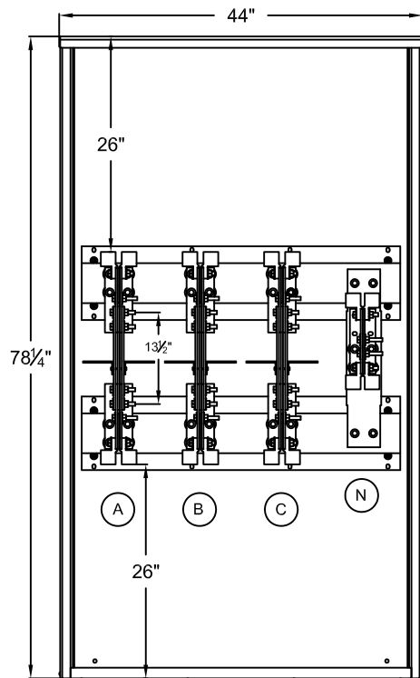
FRONT ELEVATION LESS FRONT COVERS
