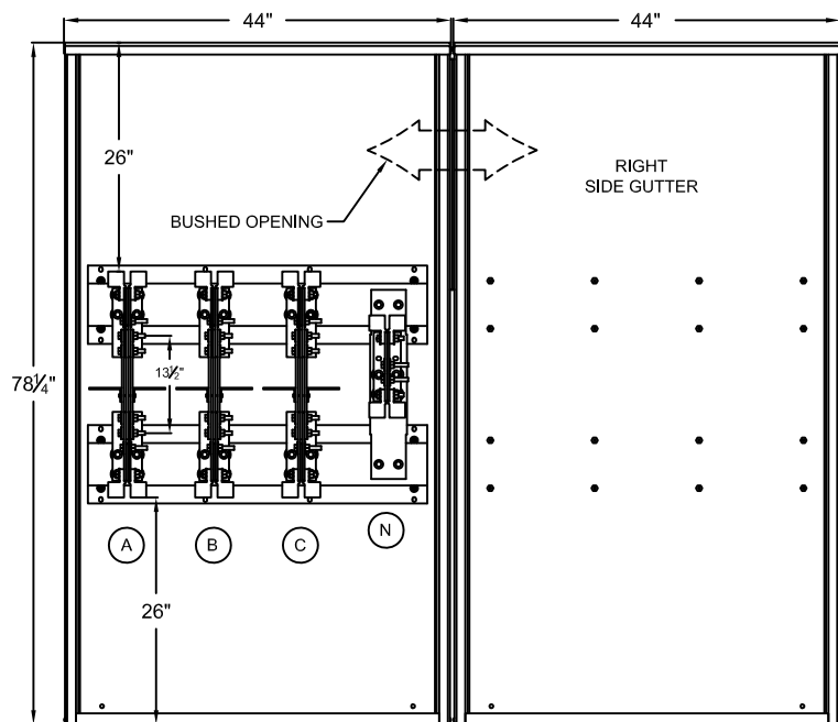
FRONT ELEVATION LESS FRONT COVERS
