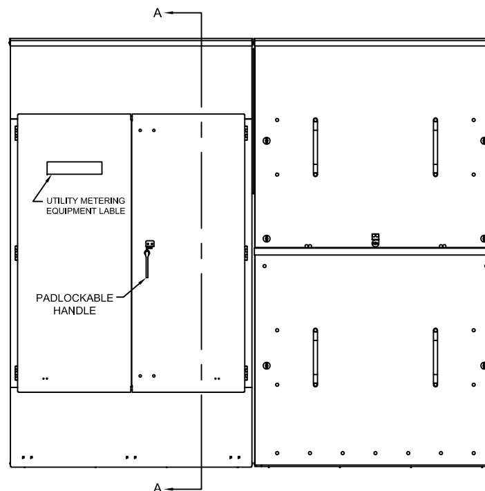
FRONT ELEVATION ENCLOSED
