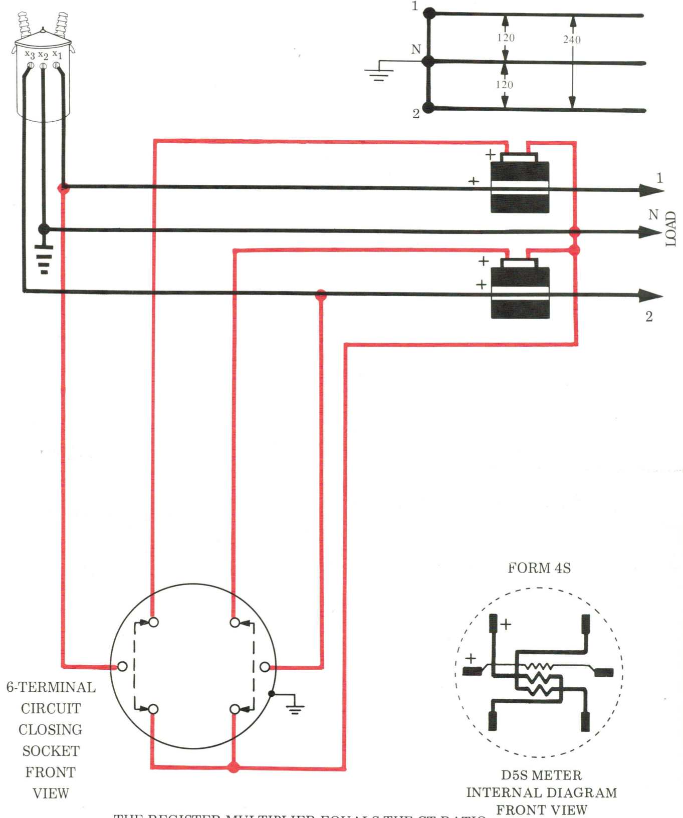
THE REGISTER MULTIPLIER EQUALS THE CT RATIO FOR SECONDARY-RATED METERS
