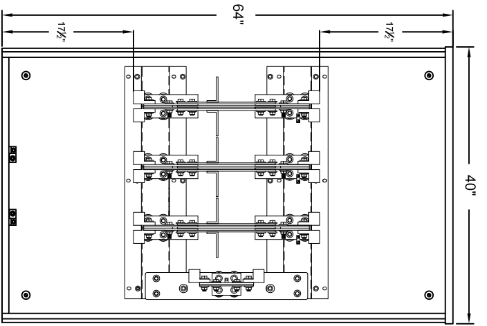
FRONT ELEVATION LESS FRONTS
