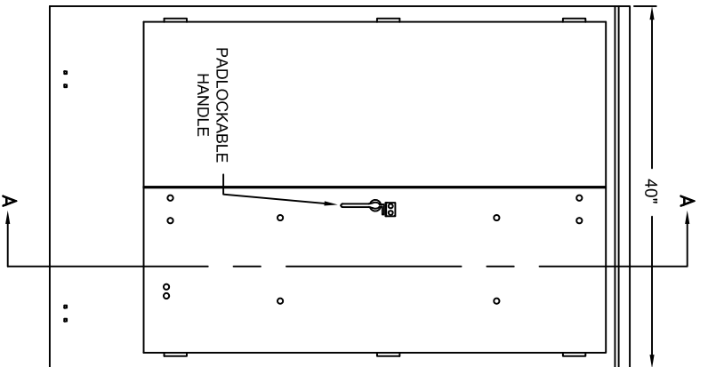
FRONT ELEVATION ENCLOSED
